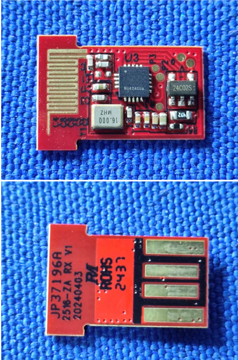
Inside View-Dongle
