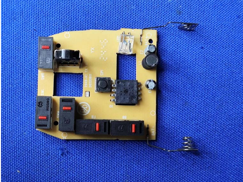
Inside View-Mouse
