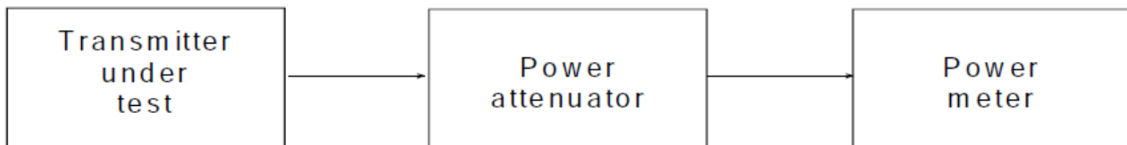
Figure 2: Measurement arrangement
