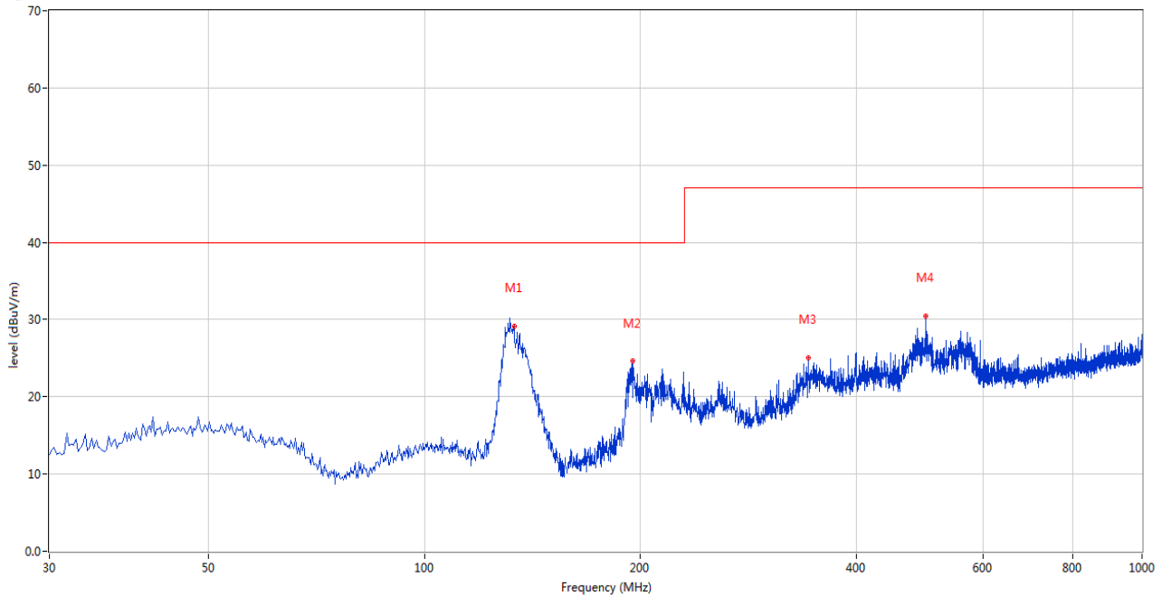
CE_EN 55032 Class B 30MHz-1GHz
